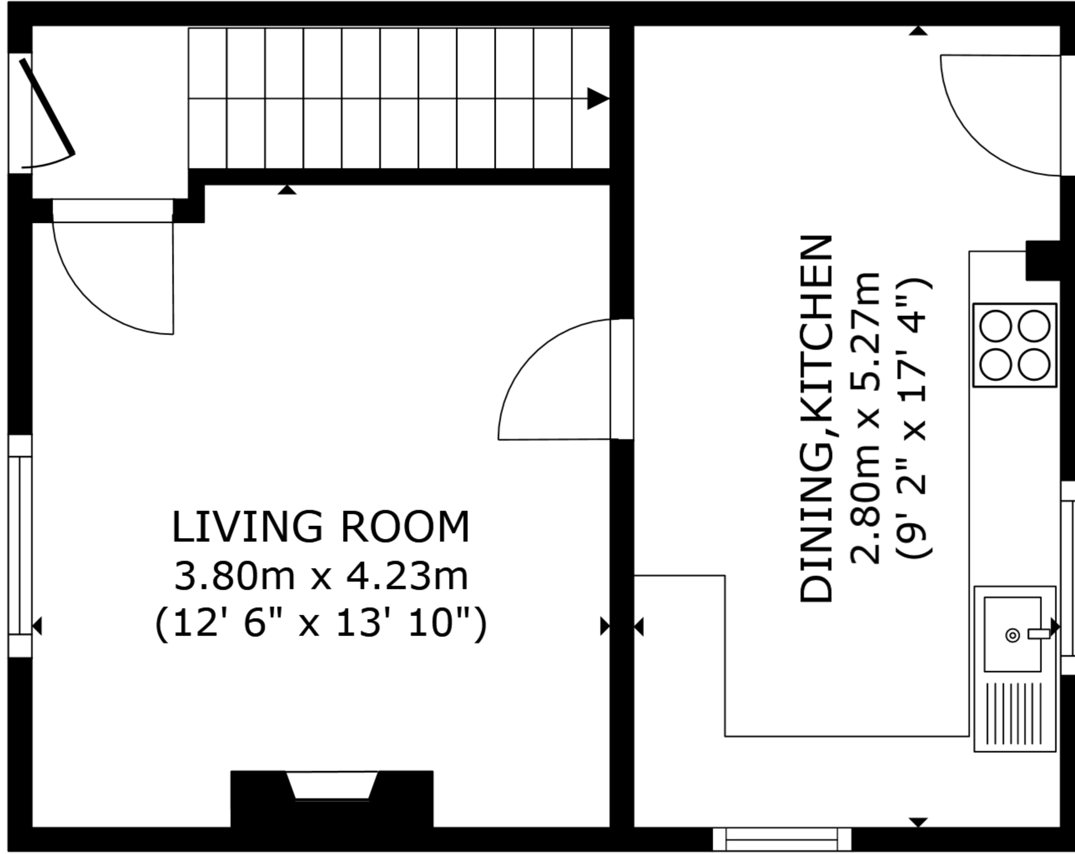
FLOOR 1
